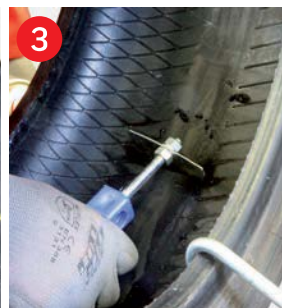
3 Clean the repair area using LIQUID BUFFER and a scraper.
