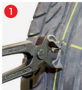
1 Locate and mark the damage. Take or screw out the foreign object.
