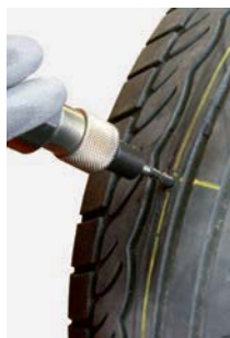
4 Prepare the puncture channel first from the tyre inside outwards, then from the outside to the inside.
